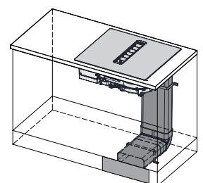
Under the plinth to-the-room outlet installation
